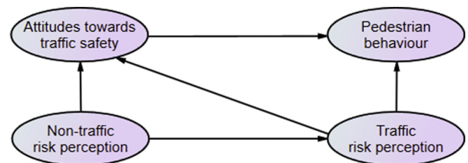
Fig. 1. A conceptual model to represent the hypothesized relationship between attitudes towards traffic safety, risk perceptions and pedestrian behaviours.
