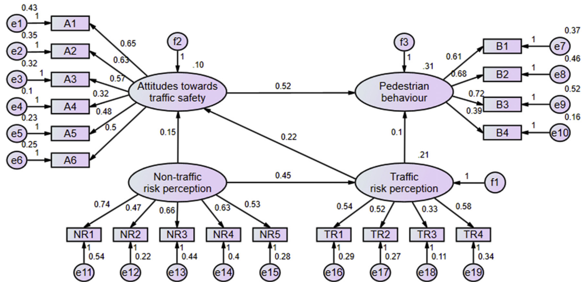
Fig. 2. Structural equation model of the relationships between attitudes towards traffic safety, traffic risk perception, non-traffic risk perception and pedestrian behaviour ( \chi^2/df = 4.30 , p < .001 ( n = 835 ), RMSEA = 0.063, CFI = 0.841, GFI = 0.924, AGFI = 0.901).
