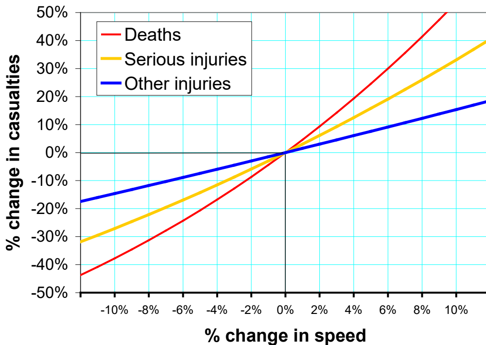
Figure 4.1: Relationship speed changes and changes in casualty rates
