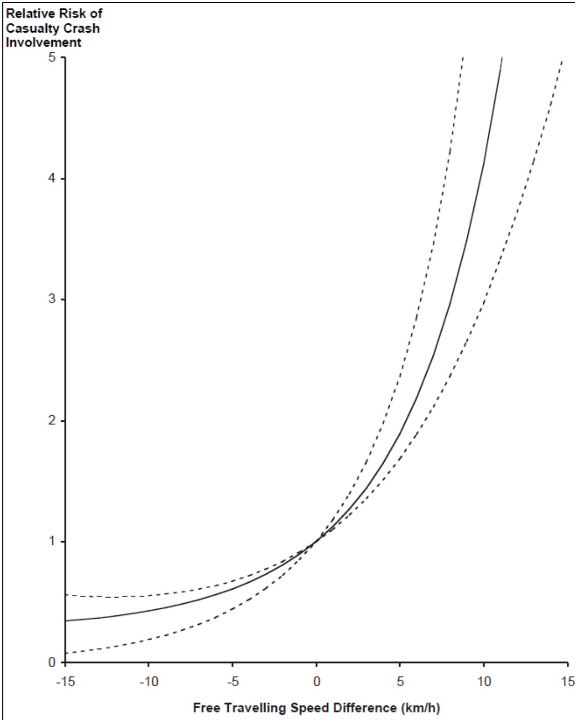
Figure 4.3: Risk of being involved in a casualty crash relative to the average control speed for a given crash site
