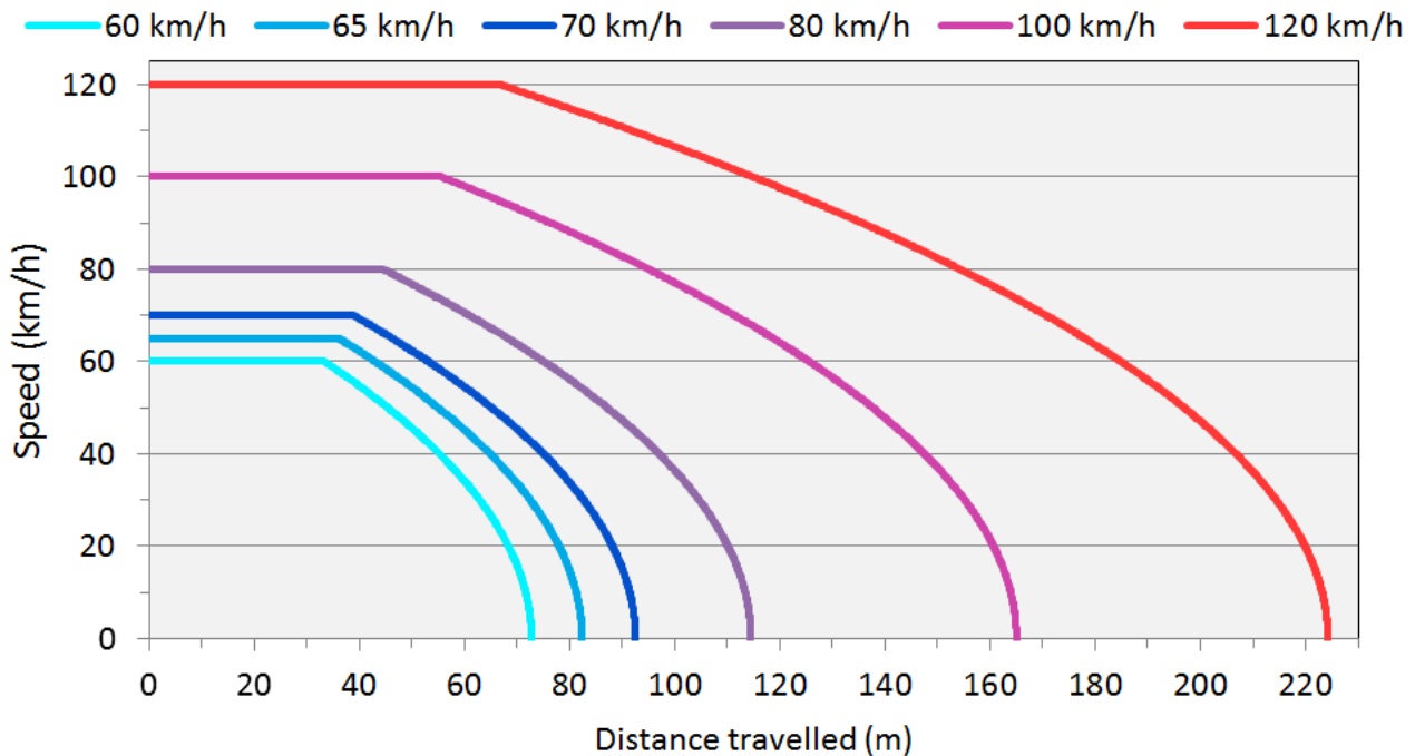
Figure 2.3: Speed versus distance travelled for vehicles travelling at different initial speeds before braking on a wet sealed pavement surface*
