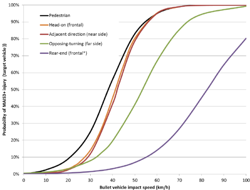
Figure 2.7: Relationships between bullet vehicle impact speed and probability of a MAIS 3+ injury to a target vehicle occupant for different crash configurations
