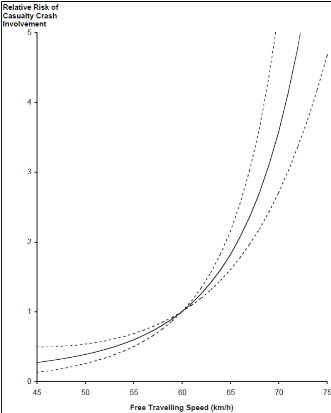
Figure 4.2: Risk of being involved in a casualty crash relative to travelling at 60 km/h in a 60 km/h speed limit zone
